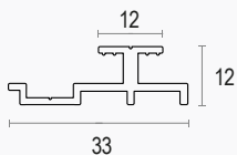
Aluminum clip AF610
