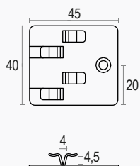
Stainless steel dual-purpose clip for Classic cladding AF611
