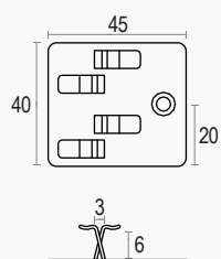
Clip AF607 for Classic flooring double use
