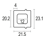
Spacer/Finishing post
