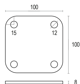
Bolt down plate
