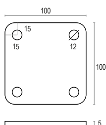
Bolt down plate for fencing H 1000 - 1200 - 1400
