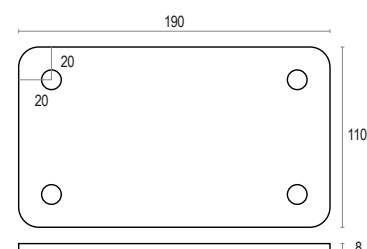
Bolt down plate for fencing H 1600 - 1800 - 2000
