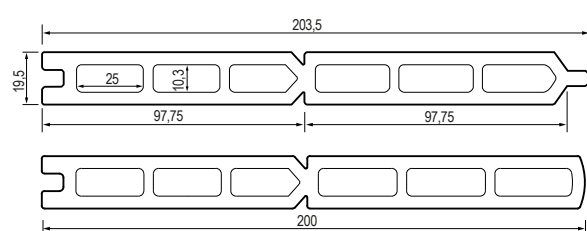
Co-extruded slats Normal and rounded
