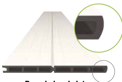
Rounded end slat Closes top part of fencing
