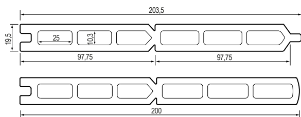
Co-extruded slats Normal and beveled
