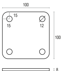
Doweling plate for fences H 1000 - 1200 - 1400
