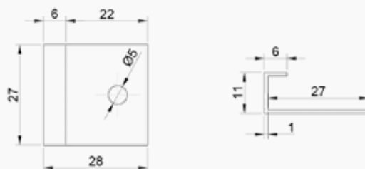
START CLIP (dimensions in mm)
