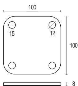
Anchor plate
