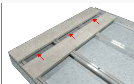
6) Lay the second slat parallel to the first and insert it into the clips
