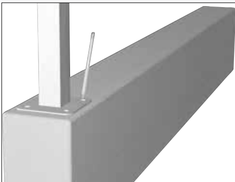
Place the initial post on the base and mark the holes on the concrete slab or curb.
