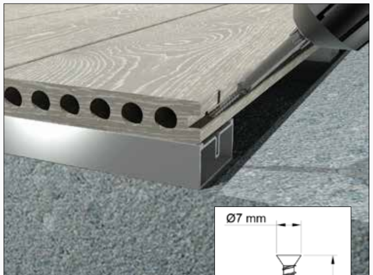
4) Insert the locking screw in the just created hole
