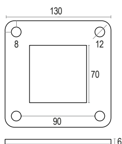
Aluminum column plate
