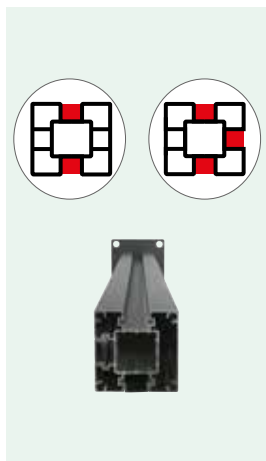
COMPLETE ALUMINUM COLUMN 2 OR 3 SLOT complete with plate, plastic cap, aluminum profile for third slot closure
