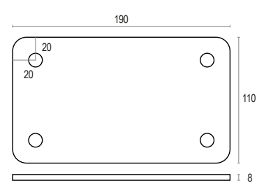
Anchor plate for fences H 1600 - 1800 - 2000
