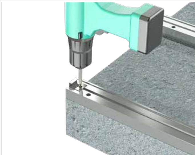
2) Apply the screw to the clip fixing it to the joist
