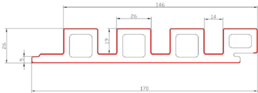
Cladding slat wood effect
