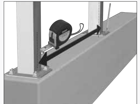
Measure the position of the next galvanized post (from column center to column center).
