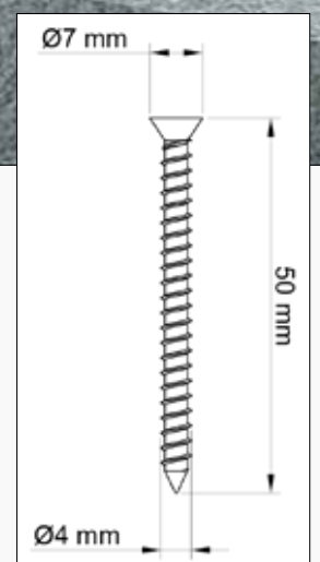
4) Insert the locking screw in the just created hole
