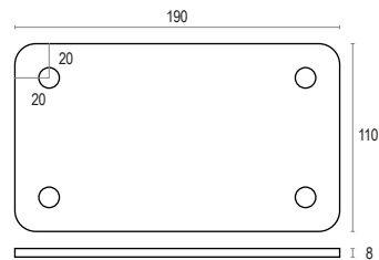
Doweling plate for fences H 1600 - 1800 - 2000
